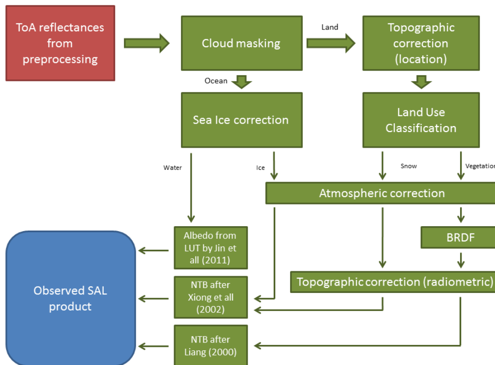
Figure 3-2: The process flow of the CLARA-A2.1-SAL product computation.
