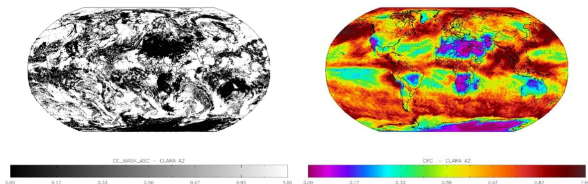
Figure 5-1: Left: Global map of CLARA-A2.1 level-2b cloud mask (0: clear; 1: cloudy) for 2008/06/21. Right: Global map of CLARA-A2.1 monthly mean total cloud fraction for 2008/06.
