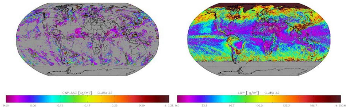
Figure 5-4: Left: Global map of CLARA-A2.1 level-2b cloud water path (in all cloud pixels) for 2008/06/21. Right: Global map of CLARA-A2.1 monthly mean liquid water path for 2008/06.
