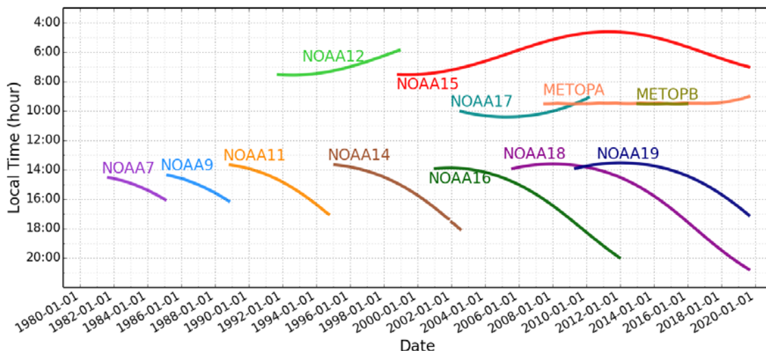
Figure 3-1: Local solar times at equator observations for all satellites from NOAA-7 to NOAA-19 and METOP A/B. Shown are all data that are used for the processing. The figure shows ascending (northbound) equator crossing times for afternoon satellites (NOAA-7 TO NOAA-19) and descending (southbound) equator crossing times for morning satellites (NOAA-12 to NOAA-17 and METOP A+B). Corresponding night-time observations take place 12 hours earlier/later. Some data gaps are present but only for some isolated dates.
