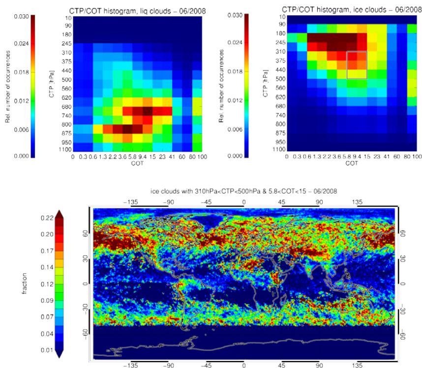
Figure 5-6: Top: Globally integrated COT-CTP histogram shown as relative frequency of occurrence for 2008/06 for liquid clouds (top-left) and ice clouds (top-right). Bottom: Global map of relative occurrence of ice clouds with CTP between 310 hPa and 500 hPa and COT between 5.8 and 15 (a indicated by the grey rectangle in the top-right plot for 2008/06).
