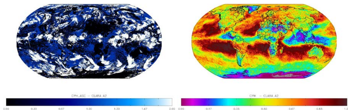
Figure 5-3: Left: Global map of CLARA-A2.1 level-2b cloud phase (0: clear; 1: liquid; 2: ice) for 2008/06/21. Right: Global map of CLARA-A2.1 monthly mean liquid cloud fraction for 2008/06.
