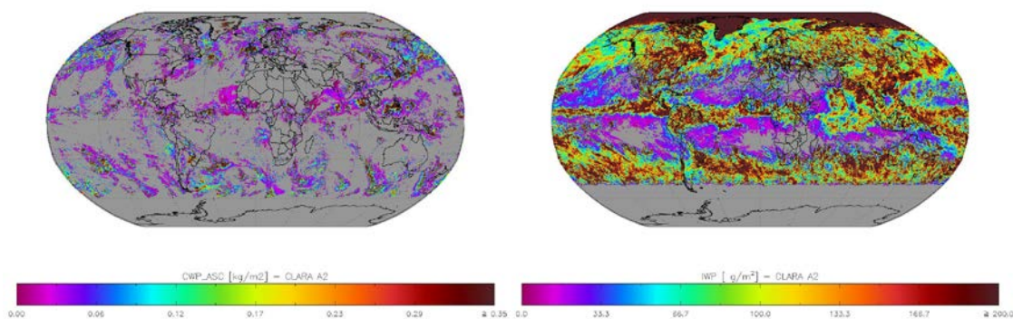
Figure 5-5: Left: Global map of CLARA-A2.1 level-2b cloud water path (in all cloud pixels) for 2008/06/21. Right: Global map of CLARA-A2.1 monthly mean ice water path for 2008/06.
