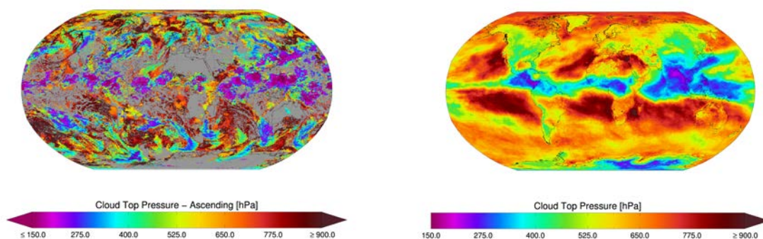
Figure 5-2: Left: Global map of CLARA-A2.1 level-2b cloud top pressure for 2008/06/21. Right: Global map of CLARA-A2.1 monthly mean cloud top pressure for 2008/06.
