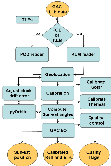
Figure 2-2: Schematic representation of the components of PyGAC interface. POD represents the satellite family that carried the second generation AVHRR instruments (i.e., AVHRR/2, up till and including NOAA-14), while KLM represents satellite family carrying the third generation instruments (AVHRR/3). PyOrbital is a part of PyTroll family of Python interfaces designed to process meteorological satellite data. (Courtesy of Abhay Devasthale, SMHI)
