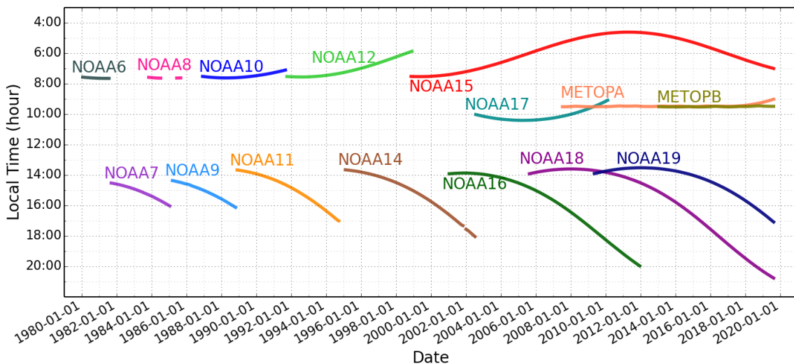
Figure 2-1: Local solar times at equator observations for all satellites from NOAA-7 to NOAA-19 and METOP A/B. Shown are all data that are used for the processing. The figure shows ascending (northbound) equator crossing times for afternoon satellites (NOAA-7 TO NOAA-19) and descending (southbound) equator crossing times for morning satellites (NOAA-12 to NOAA-17 and METOP A+B). Corresponding night-time observations take place 12 hours earlier/later. Some data gaps are present but only for some isolated dates.
