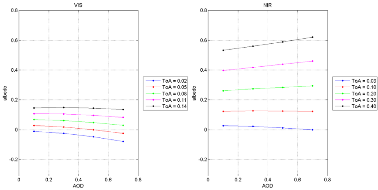
Figure 13: The sensitivity of VIS and NIR albedos of cropland on changing AOD for different TOA reflectances using SMAC with moderate angles.
