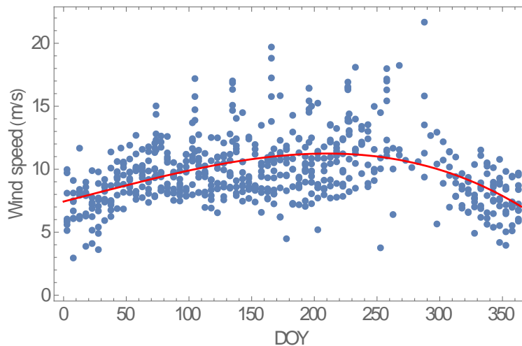
Figure 8: Variation of wind speed in one pixel during 1979-1984 and 1987-1996 as a function of the day of the year (DOY). The wind speed estimates are based on SMMR or SSM/I data. The regression polynomial (red curve) is w = 7.43593 + 0.0253204 \text{ DOY} + 0.000017422 \text{ DOY}^2 - 2.46116 \cdot 10^{-7} \text{ DOY}^3 , where w is the wind speed. This example point is situated at 60°N, 42°E.
