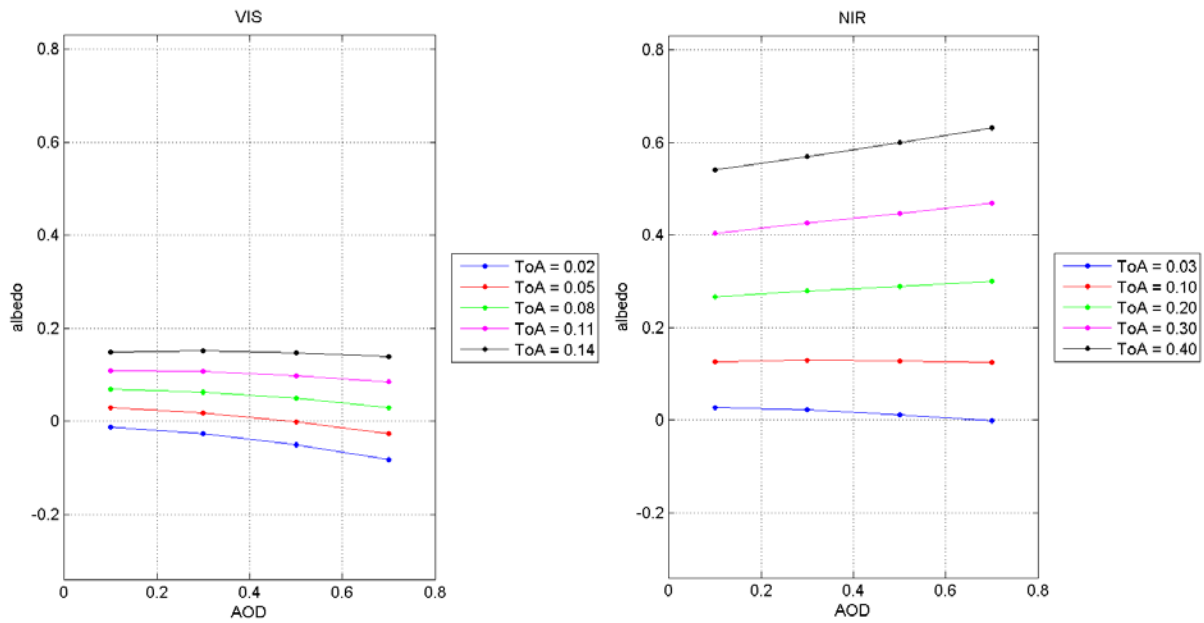
Figure 15: The sensitivity of VIS and NIR albedos of forest on changing AOD for different TOA reflectances using SMAC with moderate angles.
