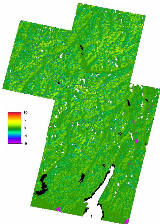
Figure 30: The difference between the flat terrain and true terrain albedo values at the Alps. The slope and aspect values were derived from ASTER DEMs and the land use
