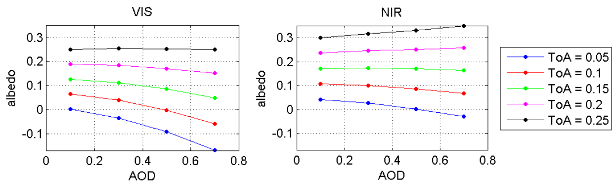
Figure 12: The sensitivity of VIS and NIR albedos of barren ground on changing AOD for different TOA reflectances using SMAC with extreme angles.
