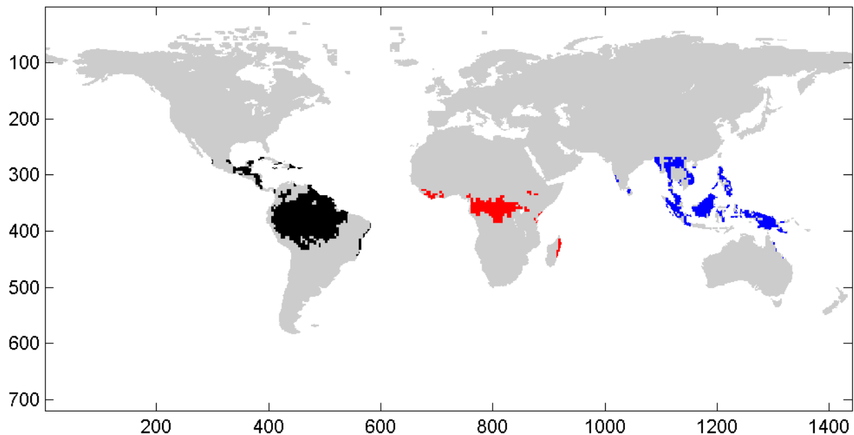
Figure 6: Example of data division using the AVHRR LUC data. The coloured areas (black, red and blue) have all the land use classification value 1 (Broadleaf Evergreen Forest). Based on the location the land use class is divided into 3 areas (marked by the different colors), which are handled separately in processing the AOD time series.
