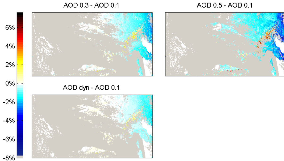
Figure 20: The absolute change in SAL albedo values in Europe between 0.3->0.1, 0.5->0.1 and dynamic->0.1. The pixels without data are marked with grey.
