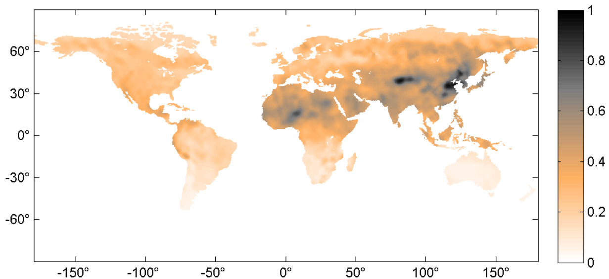
Figure 7: An example of calculated OMI-AOD on 1 st of May 2005.
