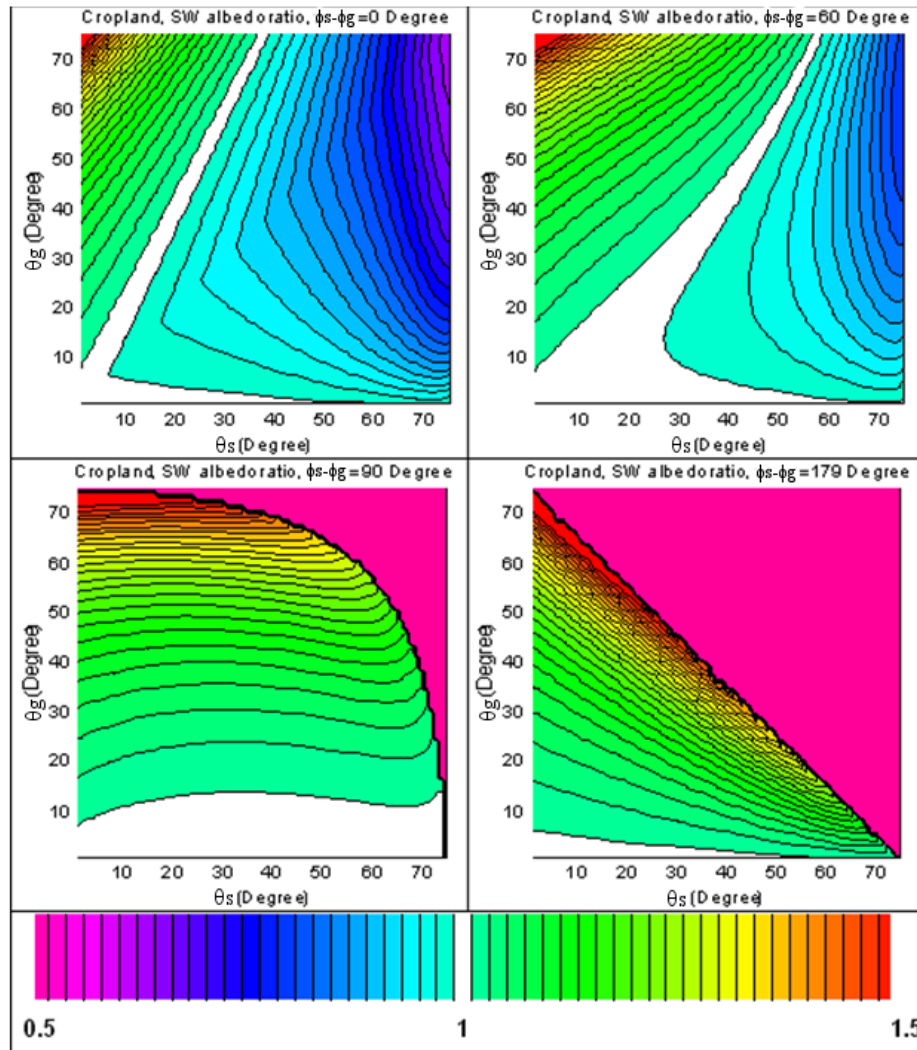
Figure 27: The ratio of the inclined and flat terrain short wave albedo of cropland for various ground ( \theta_g ) and sun ( \theta_s ) inclination angle and the azimuth angle difference ( \phi_s - \phi_g ) values. The pink shade of the images corresponding to \phi_s - \phi_g = 90^\circ and \phi_s - \phi_g = 179^\circ indicates the angle combinations, which do not contribute to the reflection at all. The lines are spaced with 2 % interval. The white area shows the parameter range producing inclined terrain albedo values matching flat terrain albedo values with \pm 1\% accuracy.
