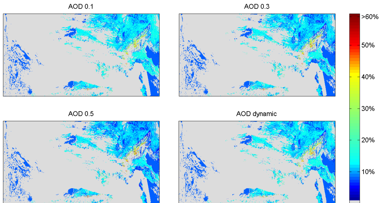
Figure 19: SAL values of Europe using AOD values of 0.1, 0.3, 0.5 and dynamic AOD. The islands of Sardinia and Corse are at the lower right corner.
