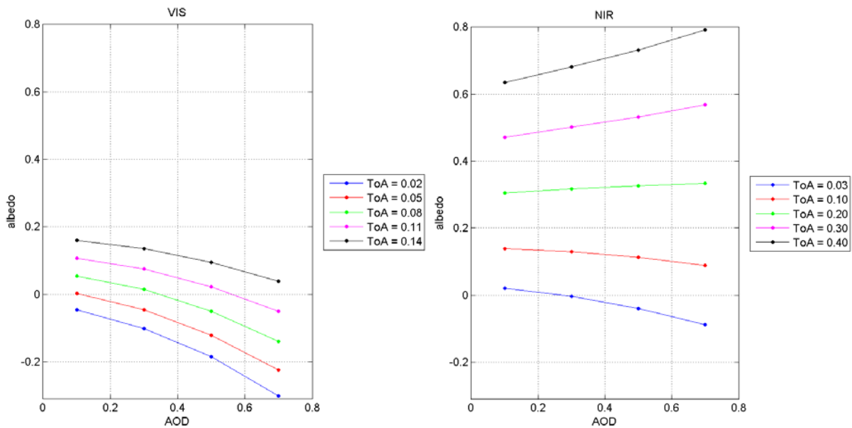
Figure 14: The sensitivity of VIS and NIR albedos of cropland on changing AOD for different TOA reflectances using SMAC with extreme angles.
