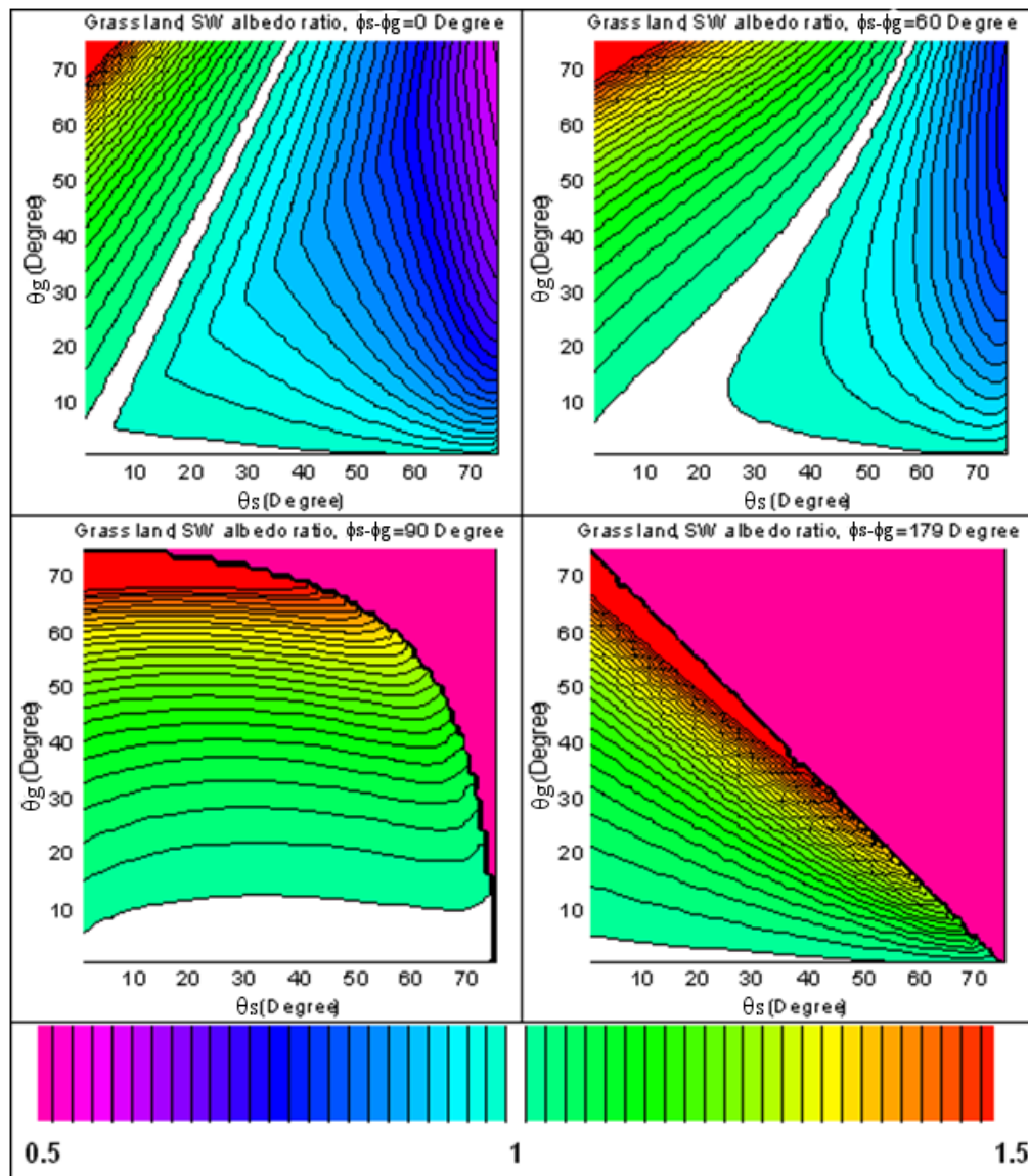
Figure 26: The ratio of the inclined and flat terrain short wave albedo of grassland for various ground ( \theta_g ) and sun ( \theta_s ) inclination angle and the azimuth angle difference ( \phi_s - \phi_g ) values. The pink shade of the images corresponding to \phi_s - \phi_g = 90^\circ and \phi_s - \phi_g = 179^\circ indicates the angle combinations, which do not contribute to the reflection at all. The lines are spaced with 2 % interval. The white area shows the parameter range producing inclined terrain albedo values matching flat terrain albedo values with \pm 1\% accuracy.
