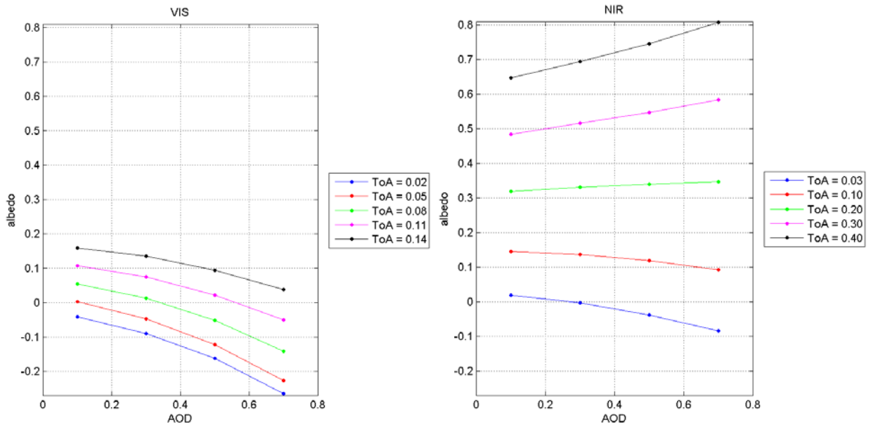
Figure 18: The sensitivity of VIS and NIR albedos of grassland on changing AOD for different TOA reflectances using SMAC with extreme angles.
