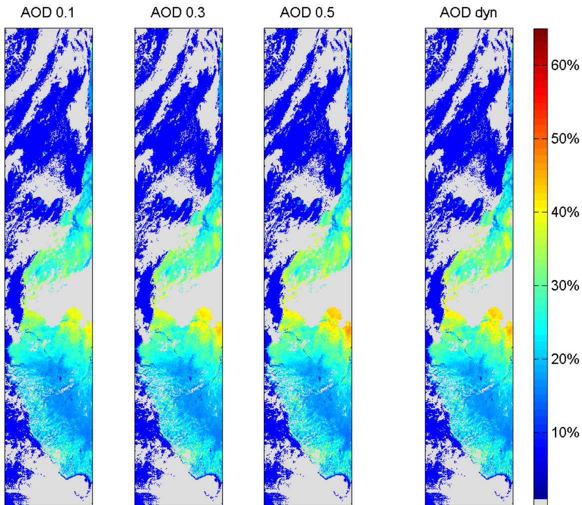
Figure 21: SAL values of North Western Africa using different AOD values. SAL value 0 represents pixels without data.
