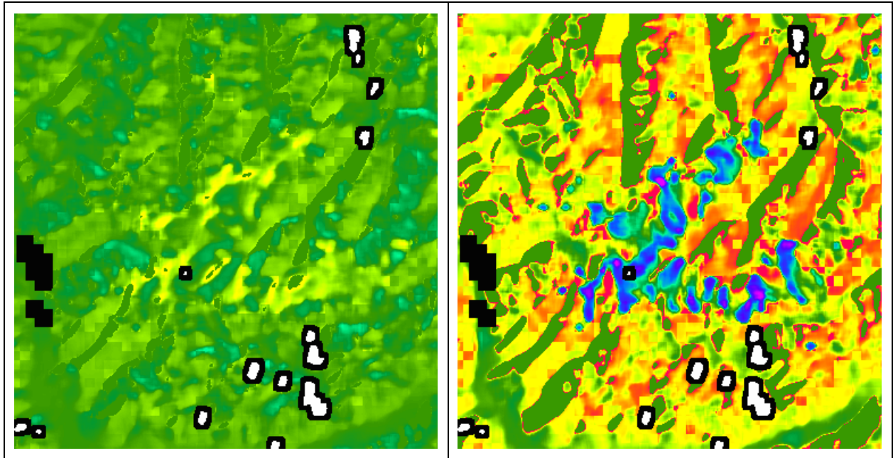
Figure 32: The difference between the flat terrain and true terrain albedo values at the Alps. A detail of Figure 30 (left) and Figure 31 (right) has been median filtered to 1 km resolution to correspond to the CLARA-SAL product. The colour code is the same as in those two Figures.
