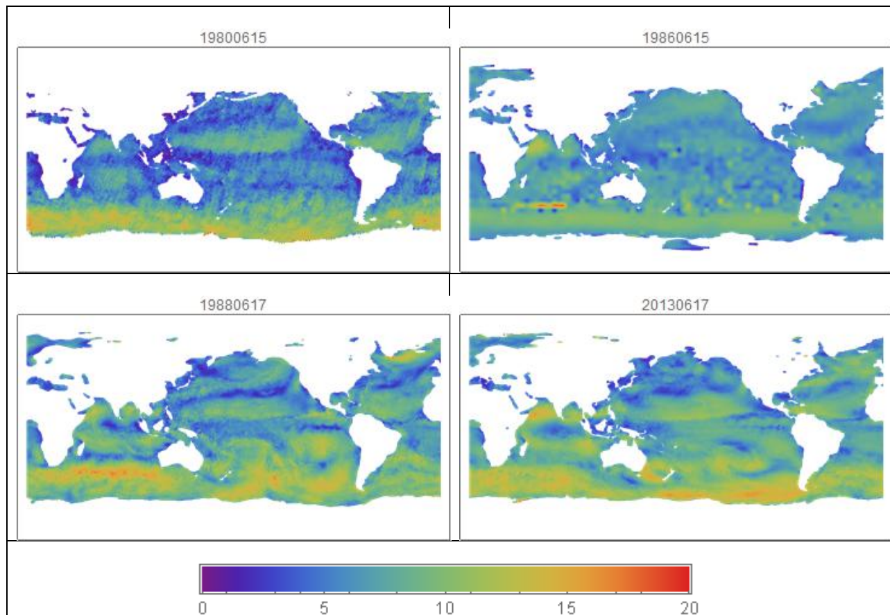
Figure 9: Wind speed examples based on SMMR (top left), anemometer (top right), SSM/I (bottom left) and SSMIS (bottom right) data. The values are in m/s.
