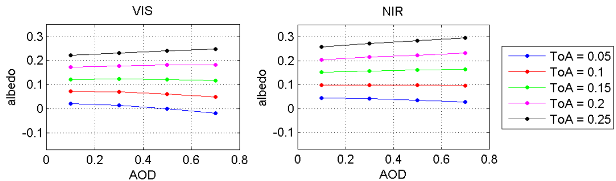
Figure 11: The sensitivity of VIS and NIR albedos of barren ground on changing AOD for different TOA reflectances using SMAC with moderate angles.
