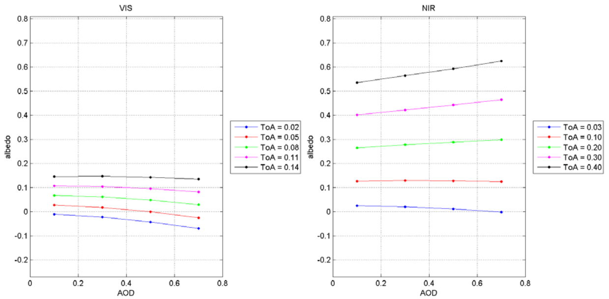
Figure 17: The sensitivity of VIS and NIR albedos of grassland on changing AOD for different TOA reflectances using SMAC with moderate angles.
