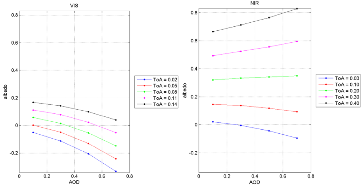
Figure 16: The sensitivity of VIS and NIR albedos of forest on changing AOD for different TOA reflectances using SMAC with extreme angles.
