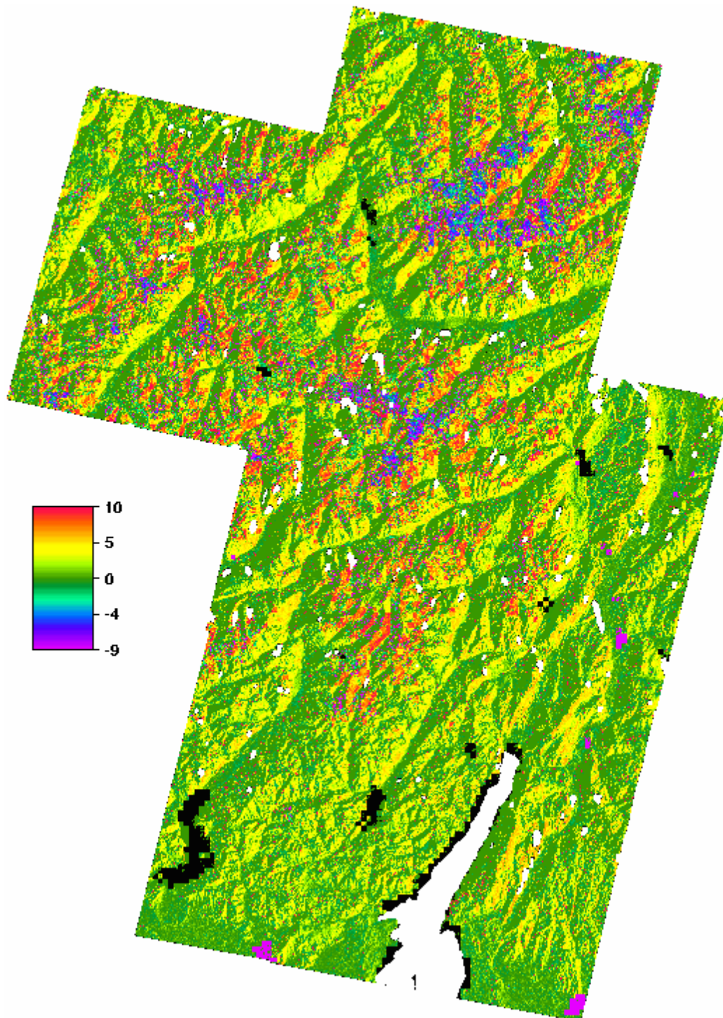
Figure 31: The difference between the flat terrain and true terrain albedo values at the Alps. The slope and aspect values were derived from ASTER DEMs and the land use
