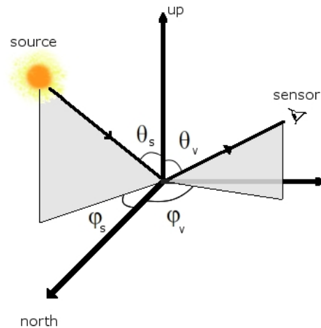
Figure 5: The BRDF geometry and relevant angles. For all non-isotropic objects, the reflectance changes as the illumination (subscript s) and viewing (subscript v) angles for elevation and azimuth change.
