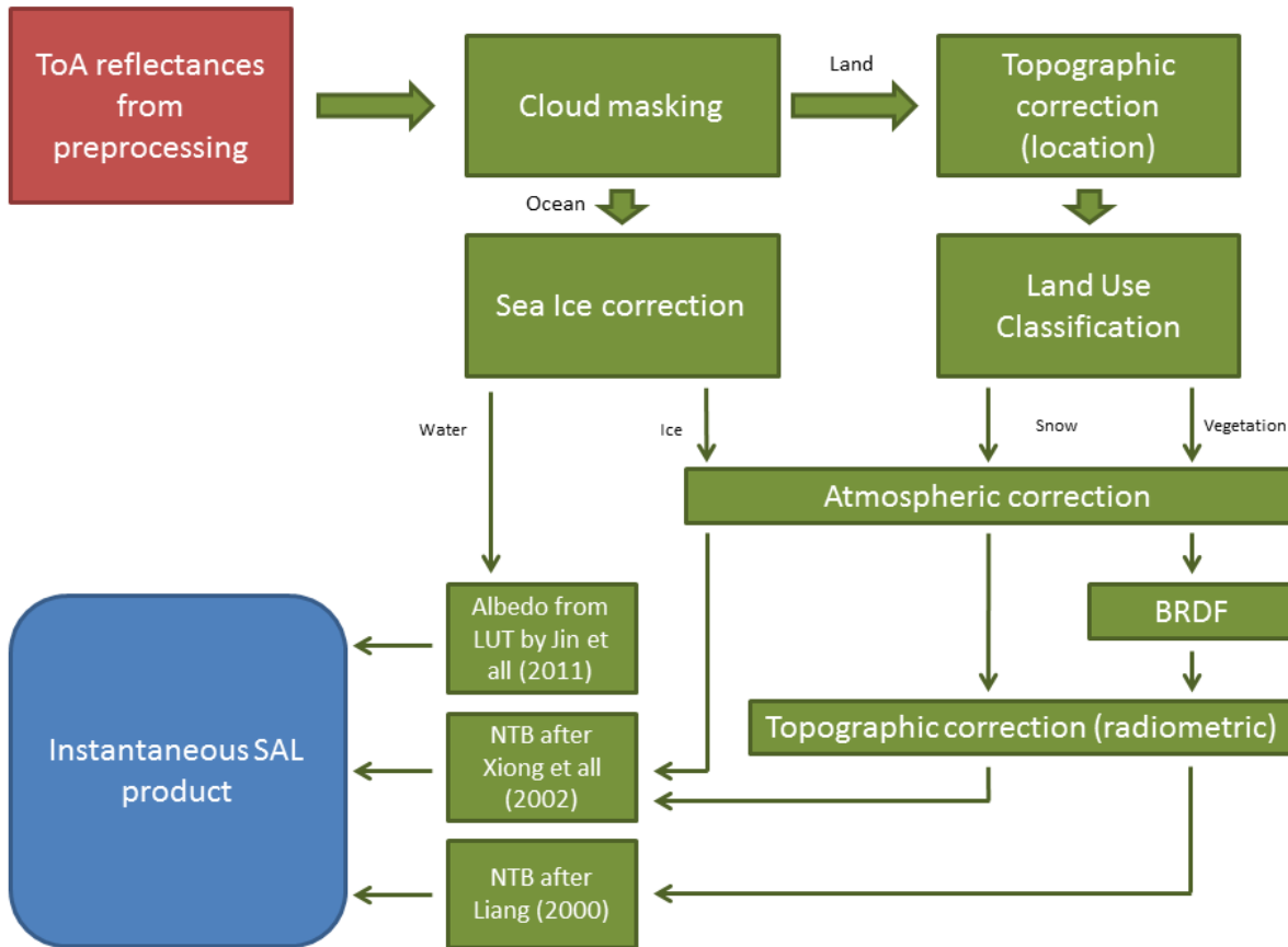
Figure 3: The process flow of the CLARA-SAL product.
