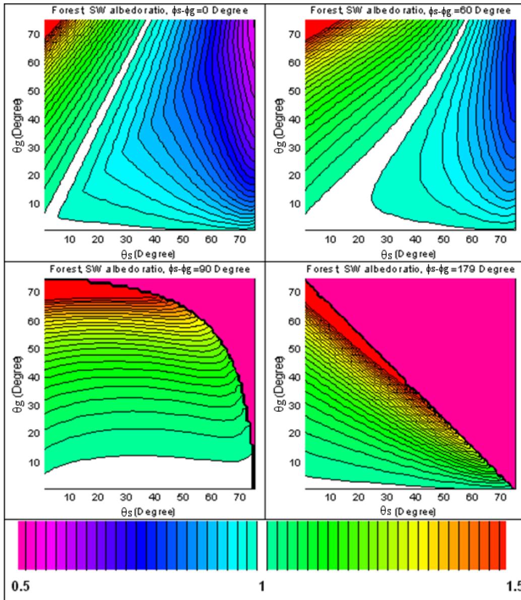
Figure 28: The ratio of the inclined and flat terrain short wave albedo of forested land for various ground ( \theta_g ) and sun ( \theta_s ) inclination angle and the azimuth angle difference ( \phi_s - \phi_g ) values. The pink shade of the images corresponding to \phi_s - \phi_g = 90^\circ and \phi_s - \phi_g = 179^\circ indicates the angle combinations, which do not contribute to the reflection at all. The lines are spaced with 2 % interval. The white area shows the parameter range producing inclined terrain albedo values matching flat terrain albedo values with \pm 1\% accuracy.
