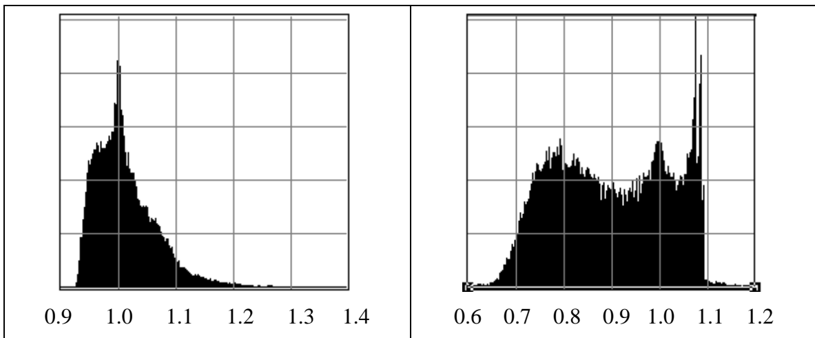
Figure 29: The histogram of the true terrain and flat terrain albedo ratio values for the Alpine test area for two sun and satellite angle cases. Left) The sun zenith angle was 31 °, the sun azimuth angle was 141°, the satellite zenith angle was 25° and the satellite azimuth angle was 181°. Right) The sun zenith angle was 70 °, the sun azimuth angle was 118°, the satellite zenith angle was 50° and the satellite azimuth angle was 181°.
