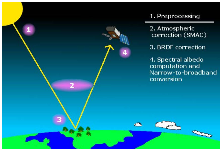
Figure 1: An illustration of the surface albedo product (CLARA-SAL) computation phases. The preprocessing is performed by Deutscher Wetterdienst (DWD) and is not a part of the actual CLARA-SAL algorithm.
