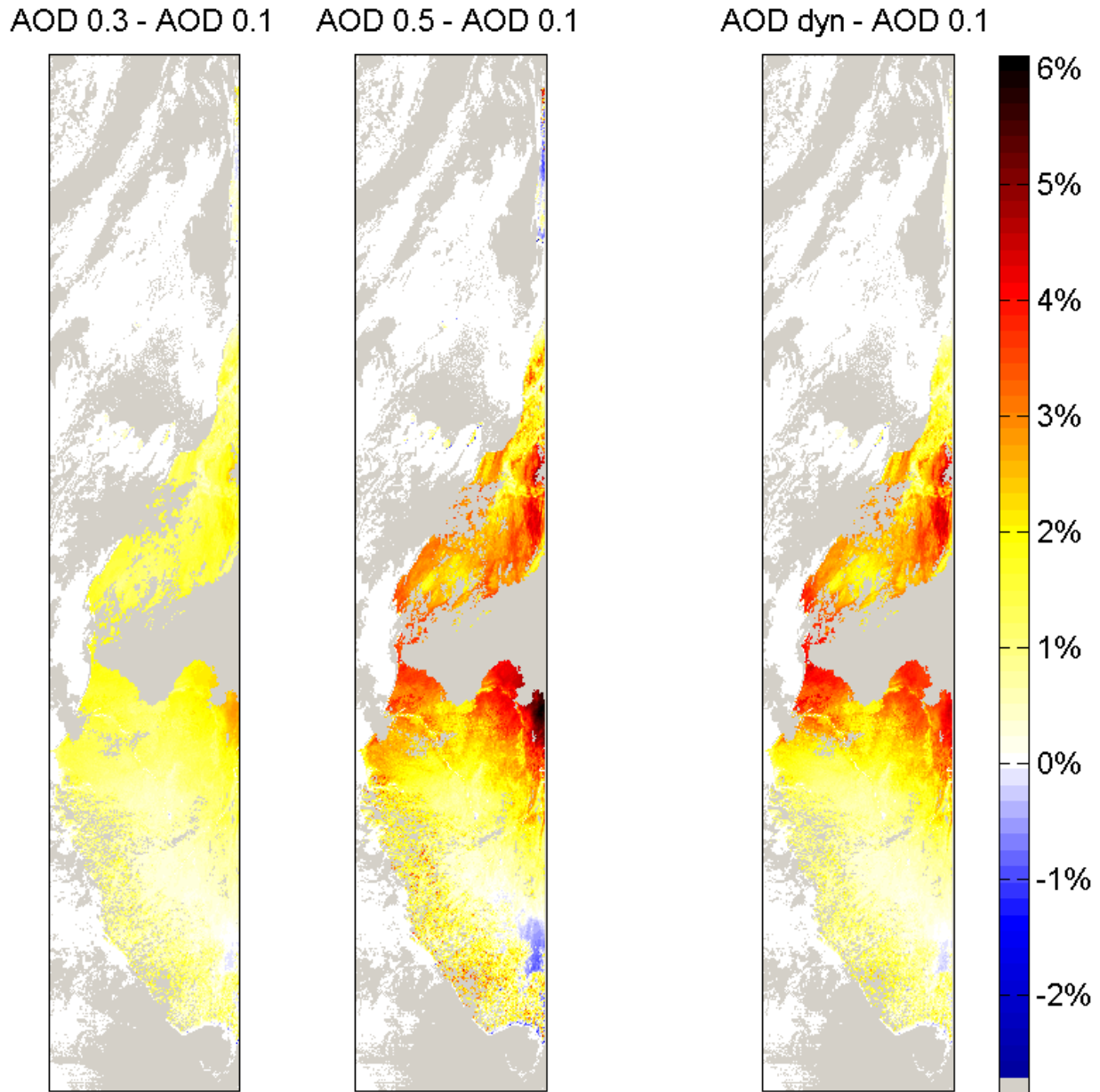
Figure 22: The absolute change in SAL albedo values between (from left to right) 0.3->0.1, 0.5->0.1 and dynamic->0.1. The pixels without data have been marked with grey.
