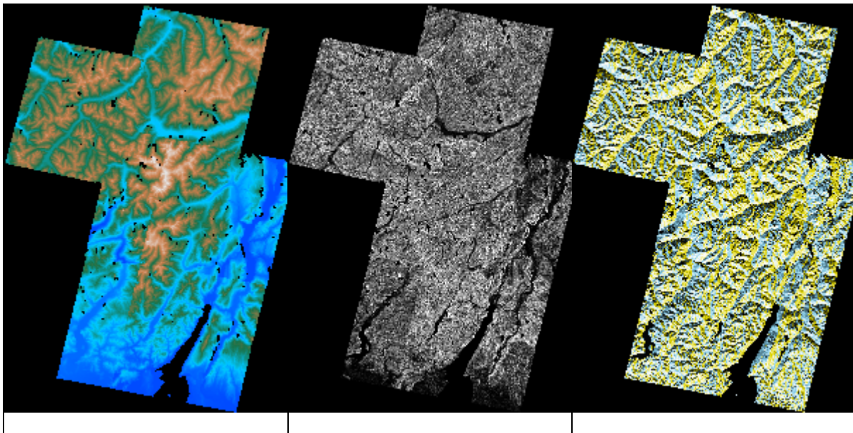
Figure 23: The ASTER DEM (left) and corresponding slope (middle) and azimuth (right) angle images from the Alps.
