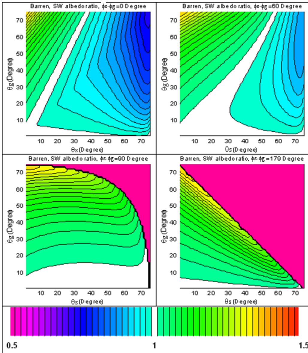
Figure 25: The ratio of the inclined and flat terrain short wave albedo of barren land for various ground ( \theta_g ) and sun ( \theta_s ) inclination angle and the azimuth angle difference ( \phi_s - \phi_g ) values. The pink shade of the images corresponding to \phi_s - \phi_g = 90^\circ and \phi_s - \phi_g = 179^\circ indicates the angle combinations, which do not contribute to the reflection at all. The lines are spaced with 2 % interval. The white area shows the parameter range producing inclined terrain albedo values matching flat terrain albedo values with \pm 1\% accuracy.
