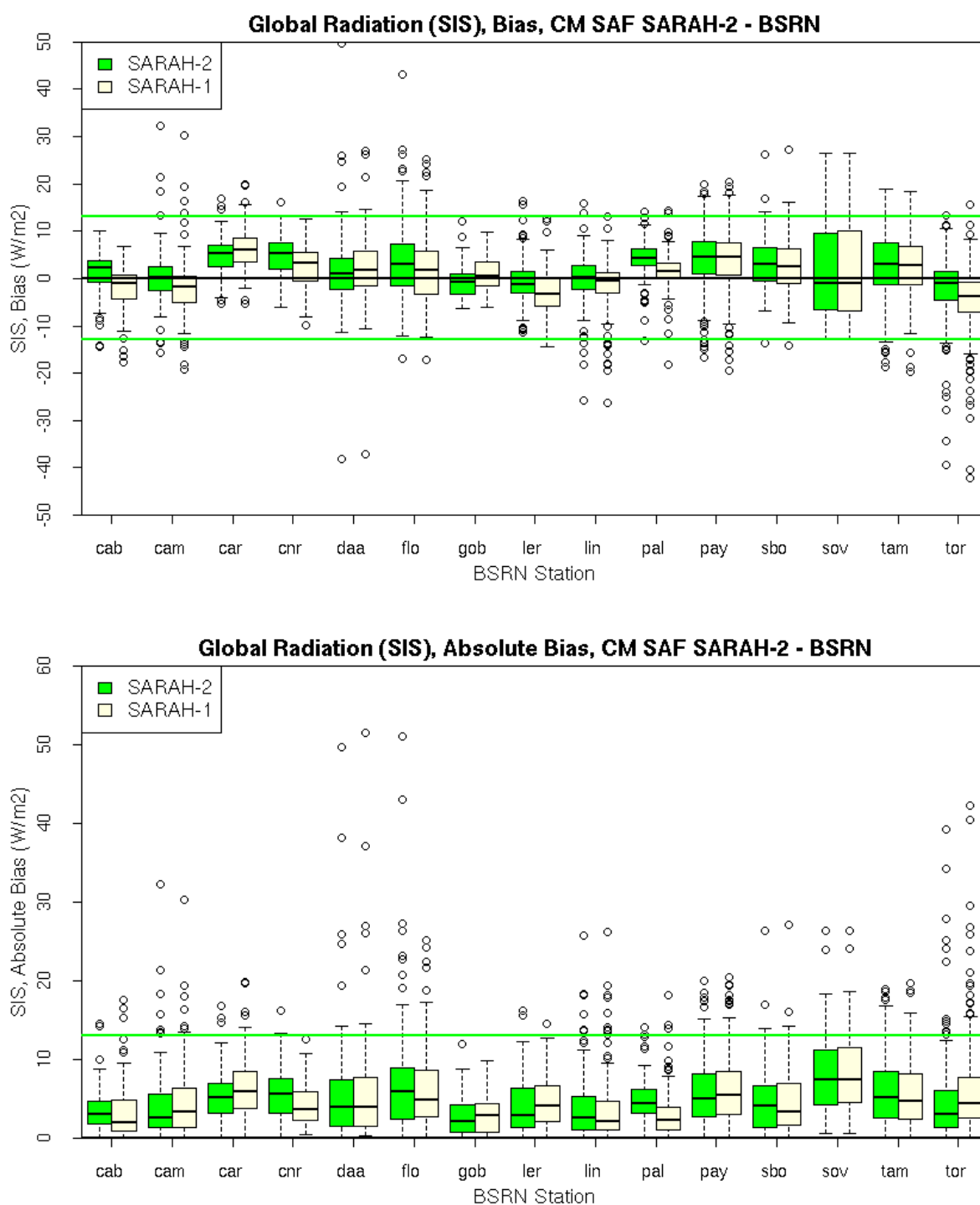
Figure 4-1: (Top) Bias and (bottom) absolute bias (MAD: mean absolute difference) between the monthly mean BSRN surface measurements and the (green) SARAH-2 SIS data record and the (yellow) SARAH-1 SIS data record for each considered BSRN station. The green lines indicate the target value of 13 \text{ W/m}^2 .
