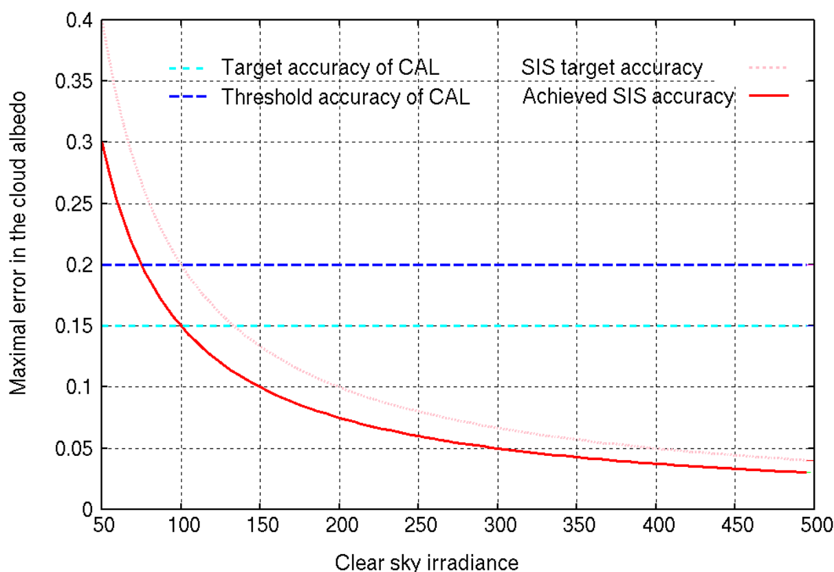
Figure 4-11: Maximal error of the effective cloud albedo (daily mean) for different clear sky irradiance values based on the derived SIS accuracy for daily means. The target accuracy is 20 W/m 2 . For the achieved SIS accuracy the mean absolute difference given in Table 4-2 has been used.
