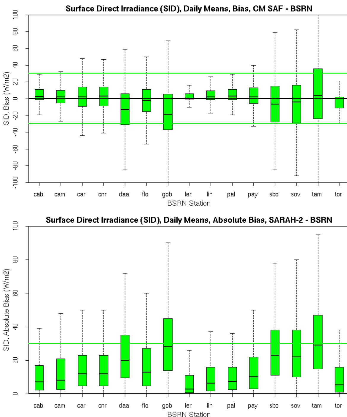
Figure 4-4: (Top) Bias and (bottom) absolute bias for the comparison of daily mean SID data between the BSRN stations and the SARA-2 Surface radiation data record. No outliers are shown here.
