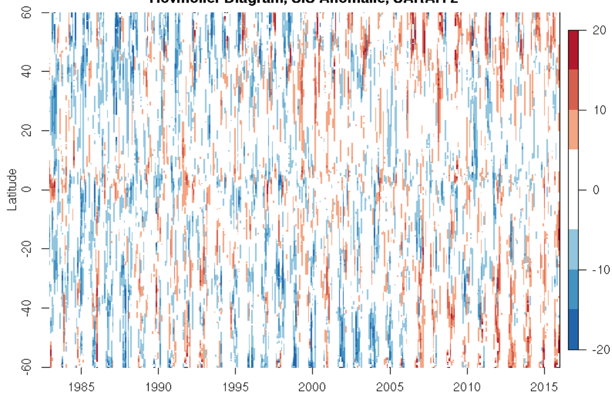
Hovmoller Diagram, SIS Anomalie, SARA-H2
