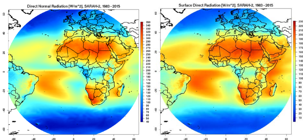
Figure 2-1: Multiyear means of SIS (top), and of the SDI Parameters DNI (bottom left) and SID (bottom right) for the SARAH-2 climate data record (1983-2015).
