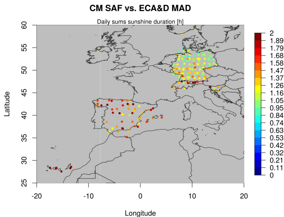
Figure 4-16: Mean absolute difference (MAD) for the comparison of sunshine duration daily sums of ECA&D station data and SARAH-2 SDU.
