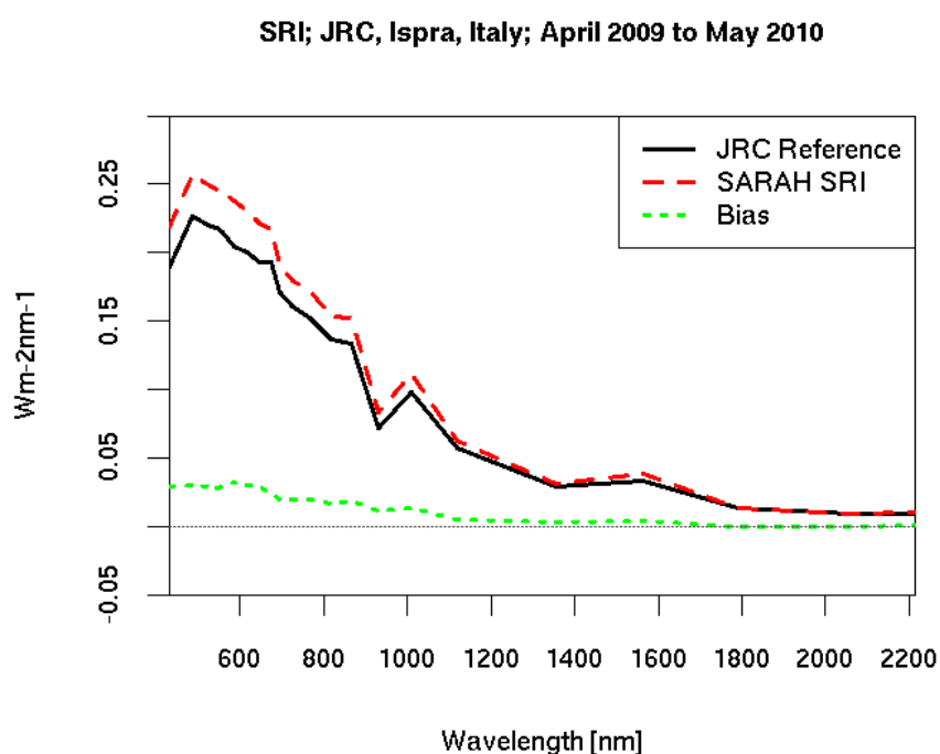
Figure 4-7: Mean Spectral Irradiance from April 2009 to May 2010 in Ispra, Italy, based on surface measurements (black line) and the SARA2 SRI data record (red dashed). The dotted green line represents the bias.
