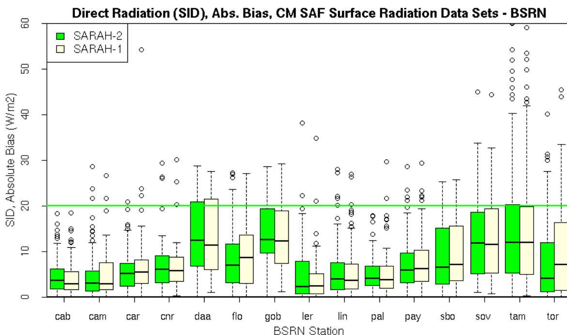
Figure 4-3: (Top) Bias and (bottom) absolute bias (MAD: mean absolute difference) between the monthly mean BSRN surface measurements and the (green) SARAH-2 SID data record, and the (yellow) SARAH-1 SID data record for each considered BSRN station. The solid green line indicates the target value of 20 W/m 2 for SID.
