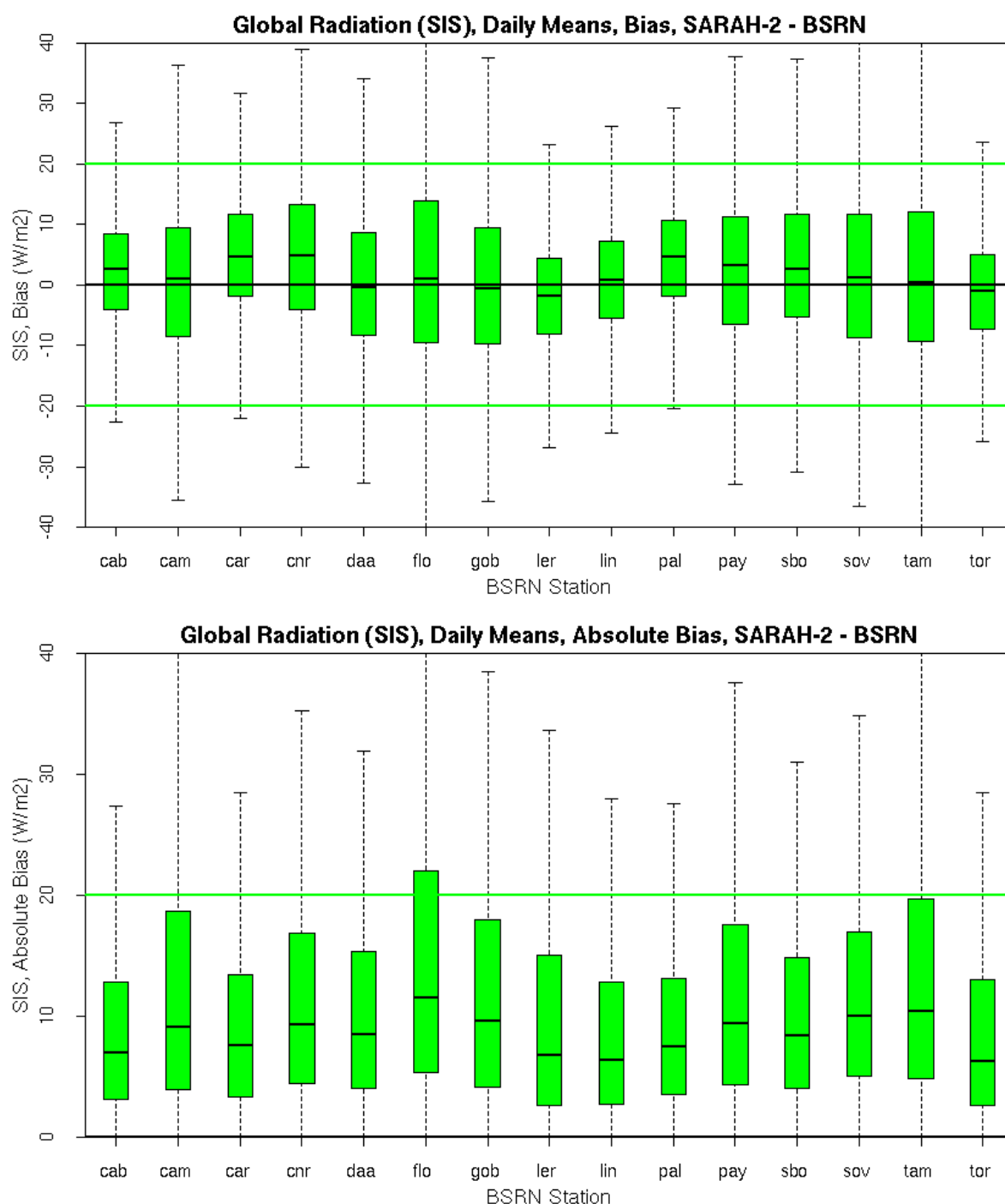
Figure 4-2: (Top) Bias and (bottom) absolute bias for the comparison of daily mean SIS between the BSRN stations and the SARAH-2 Surface radiation data record. No outliers are shown here. The green lines indicate the target accuracy for the SIS daily means.
