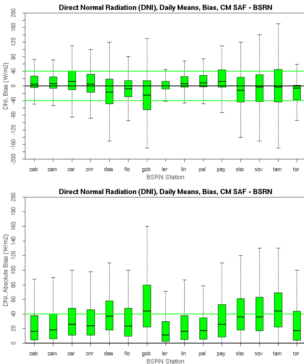
Figure 4-6: (Top) Bias and (bottom) absolute bias for the comparison of daily mean DNI between the BSRN stations and the SARAH Surface radiation data record. No outliers are shown here.
