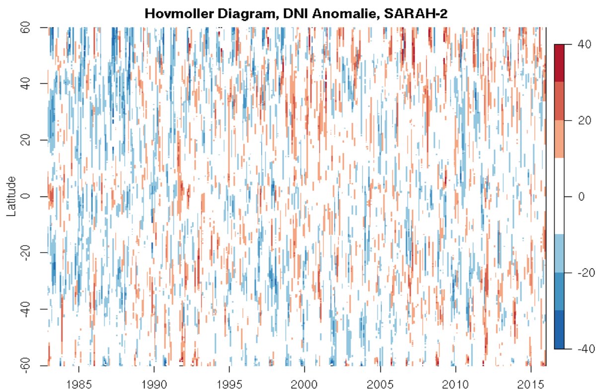
Figure 6-1: Hovmoeller diagrams of the monthly mean anomaly of (top) SIS and (bottom) DNI.
