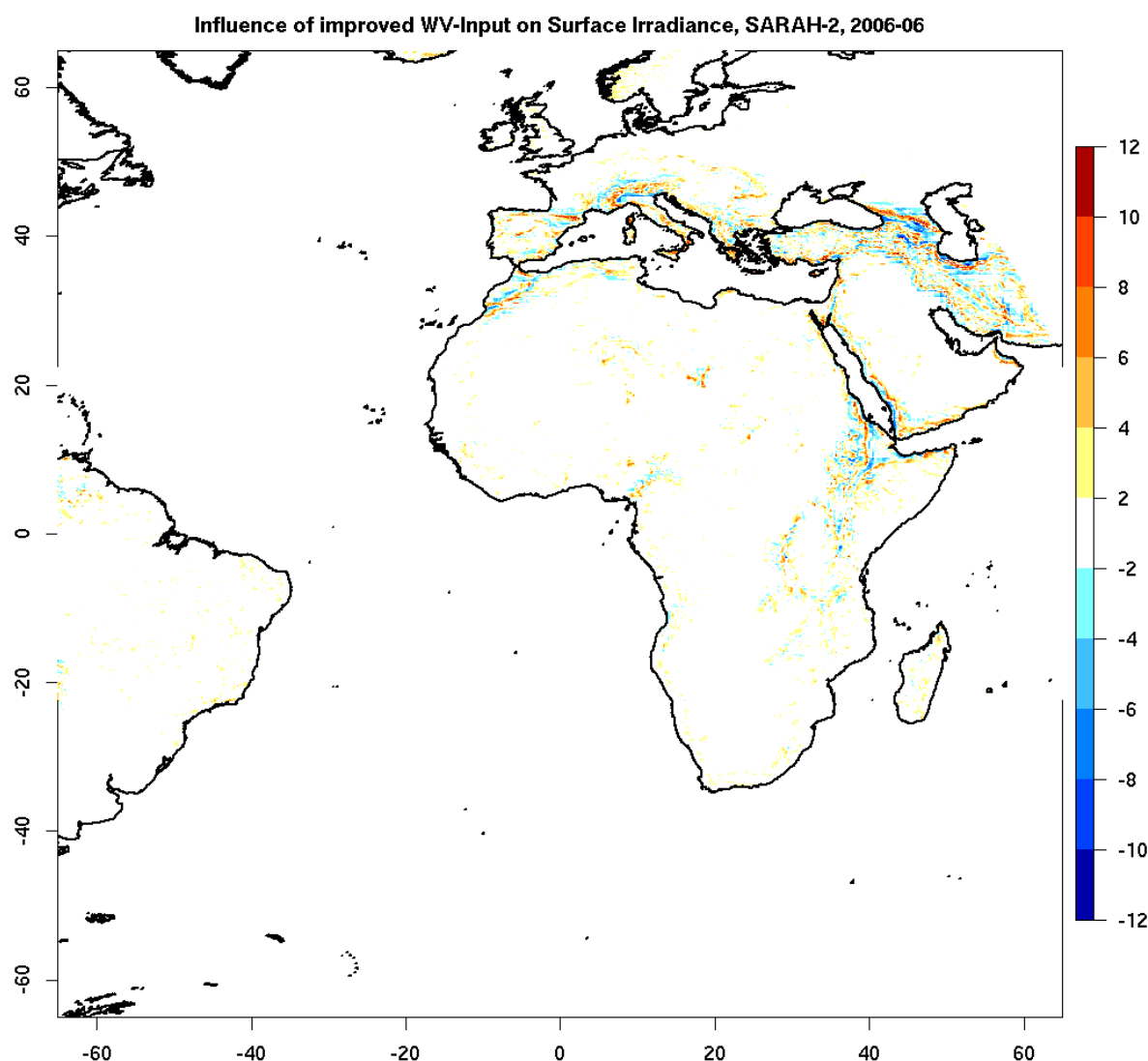
Figure 5-2: Influence of downscaled water vapor on SIS in W/m^2 for the monthly mean of 2006-06 on the full METEOSAT-disk. As in Figure 5-1, the difference SARAH-2 minus SARAH-1 is plotted.
