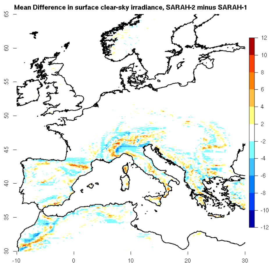
Figure 5-1: Influence of downscaled water vapor input on clear-sky radiation. The mean difference of SARA-2 minus SARA-1 clear-sky radiation is shown in W/m^2 .
