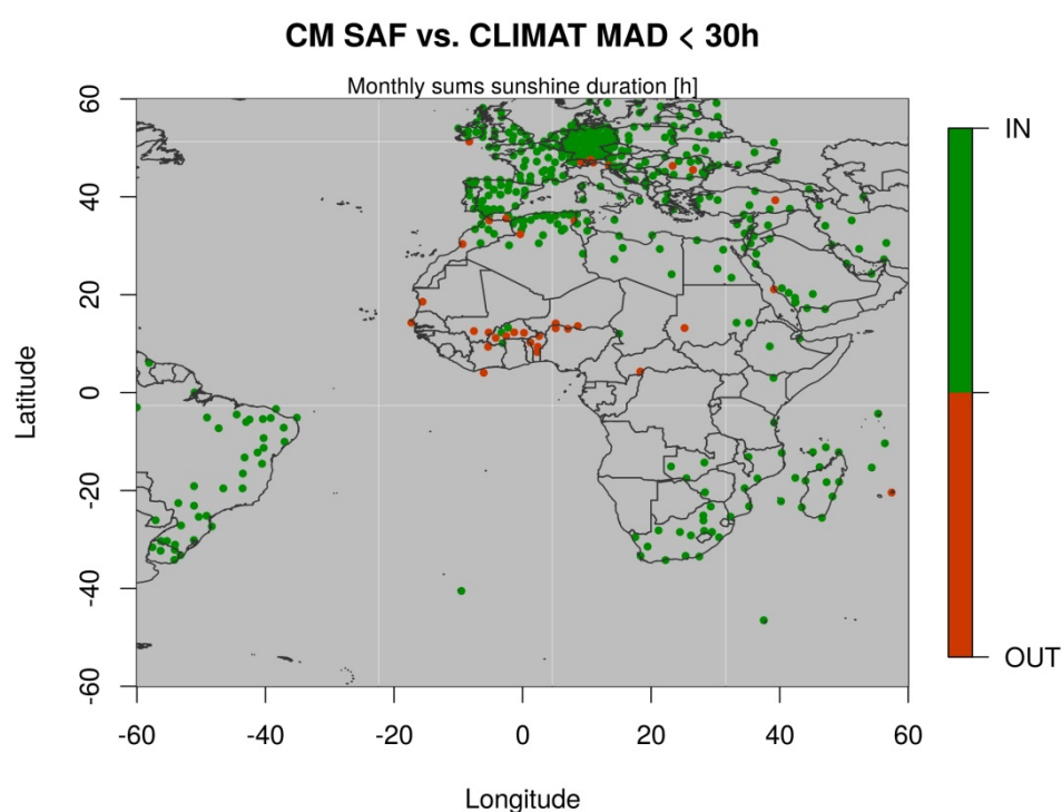
Figure 4-14: Stations matching the threshold accuracy (MAD < 30 h) for the comparison of sunshine duration monthly sums of CLIMAT station data and SARA-2 SDU.
