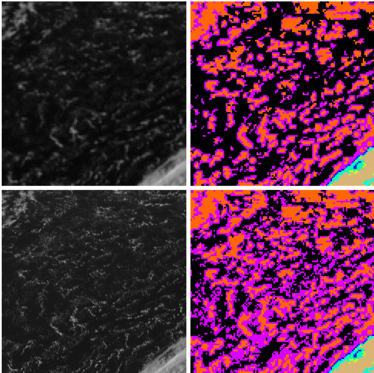
Figure 16 Shallow convection maritime clouds over Northern Atlantic, 8 September 2009. 17h00UTC, (120x120 at low resolution SEVIRI scale). Top left: 0.8 \mu\text{m} visible reflectance; top right: v2009 cloud type; bottom left: HRV reflectance; bottom right: v2010 cloud mask
