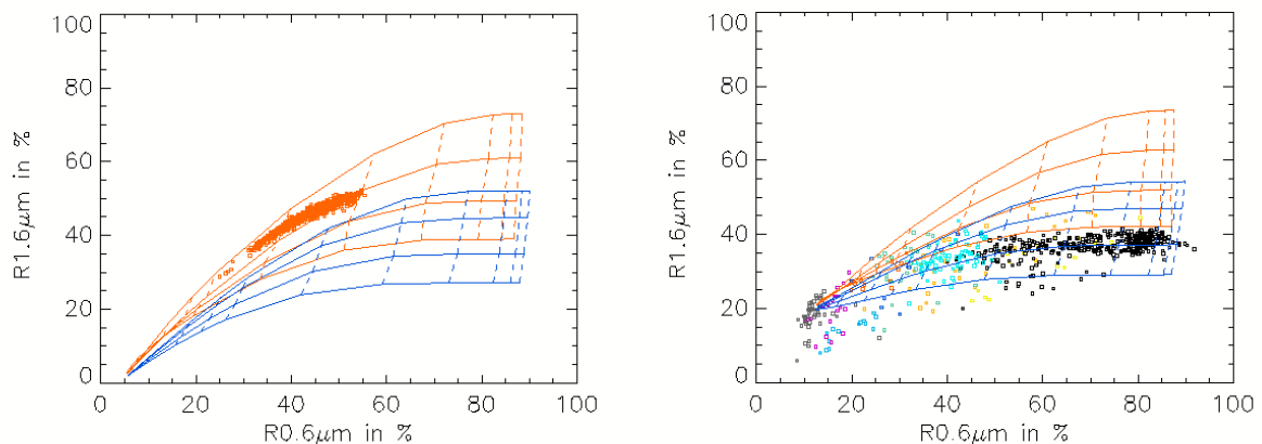
Figure 30 Illustration of the cloud phase retrieval using 0.6 \mu\text{m} and 1.6 \mu\text{m} reflectances. Cloud measurements (coloured using CT cloud type colors, except white color replaced by black) are superimposed to simulated curves. Left: for a maritime stratocumulus cloud; right: for a convective system over the Pyrenees.
