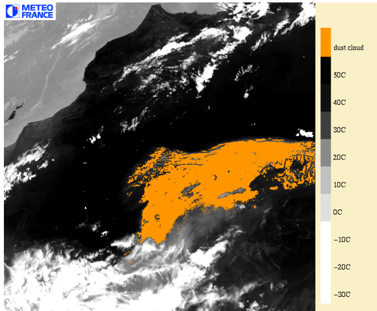
Figure 25: Example of SEVIRI dust cloud flag superimposed on a 10.8 \mu m infrared image: dust cloud over North Africa on 14 th July 2003 at 13h00 UTC.
