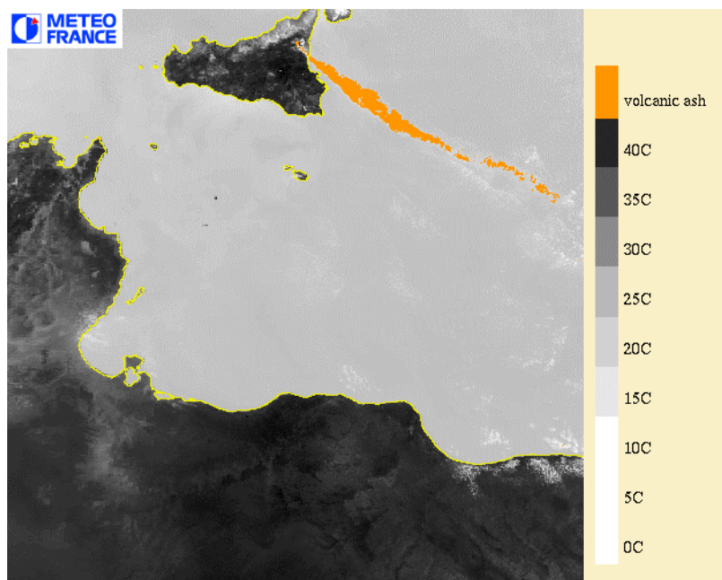
Figure 26: Example of MODIS volcanic ash cloud superimposed on a 10.8 \mu m infrared image: Etna eruption on 22 th July 2001 at 9h55 UTC.
