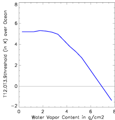
Figure 6: Illustration of T_{12.0T3.9\text{threshold}} over the Ocean for a satellite zenith angle of 48 degrees.
