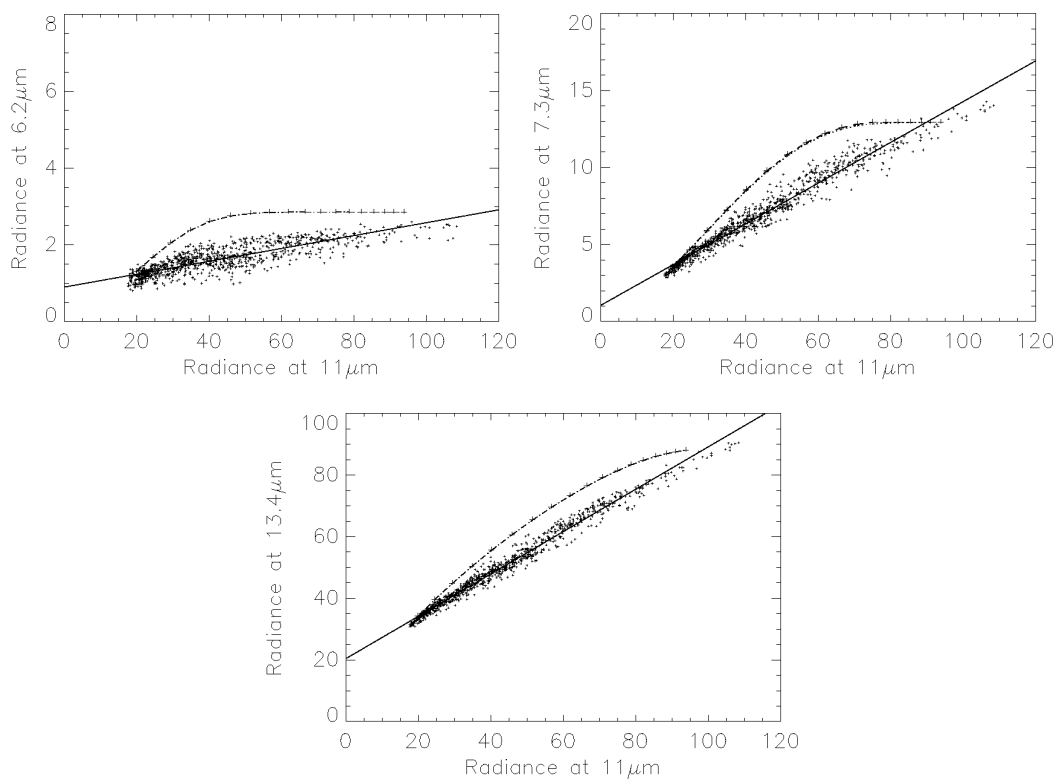
Figure 35: Illustration of the H 2 O/IRW intercept method with SEVIRI radiances (expressed in \text{mWm}^{-2}\text{sr}^{-1}\text{cm} ).
