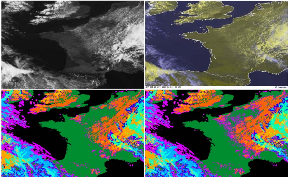
Figure 18 Fair-weather cumulus in subsident air over western Europe, 23 June 2009, 14h00UTC, (1270x770 at SEVIRI low resolution scale). Top left: enhanced 0.6 μm visible reflectance; top right: EUMETSAT RGB (12-12-9); bottom left: v2009 cloud type; bottom right: v2010 cloud type
